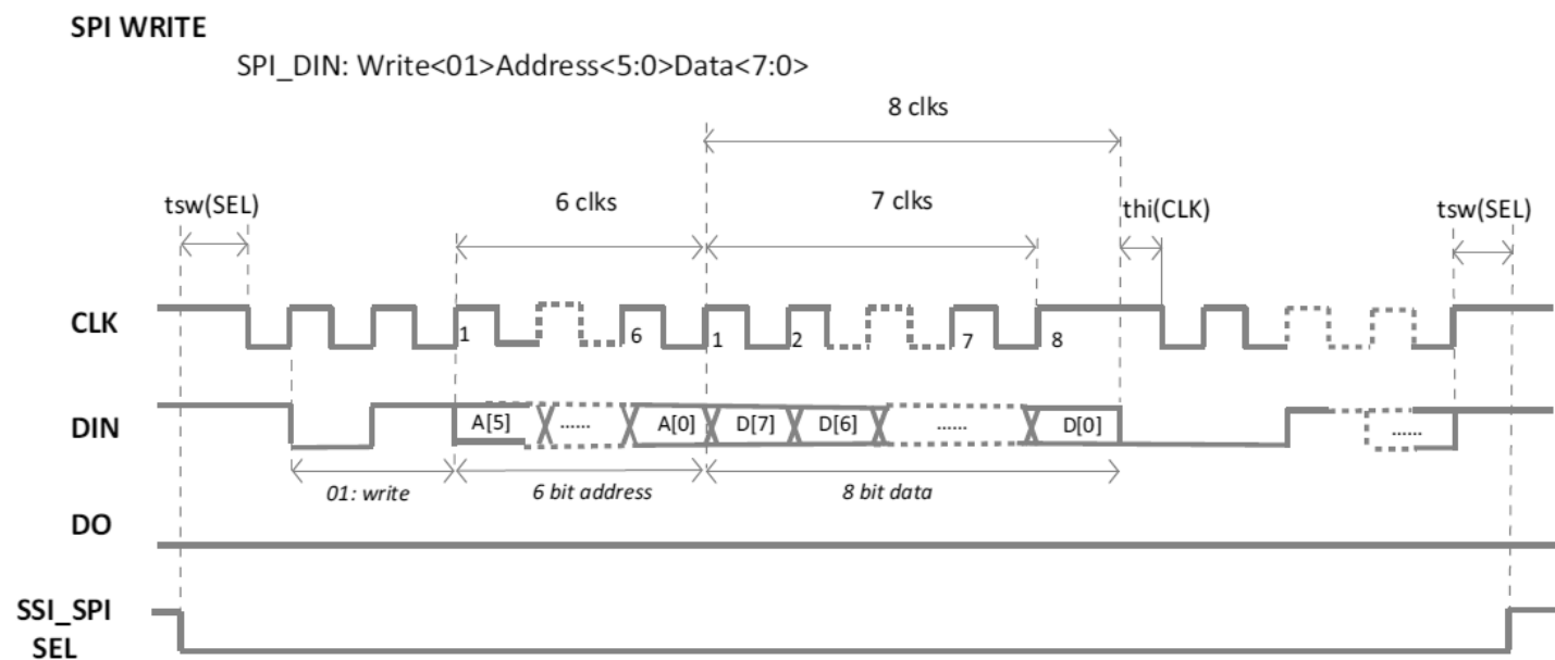
Figure 15: SPI Write Timing Diagram
